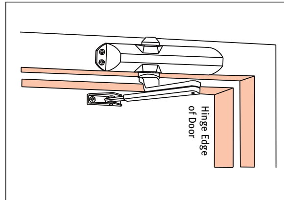
Top Frame Fixing (Fig. 2)
